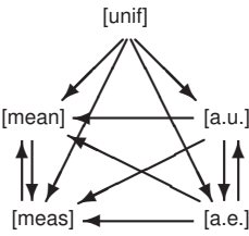
Figure 4.2: Comparison of modes of dominated convergence.
